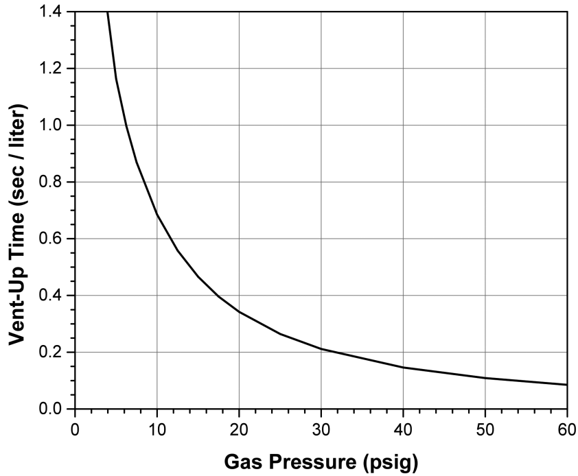
Mott GSE-FLG-0.6-2.5-F1-NW25 Performance Data
