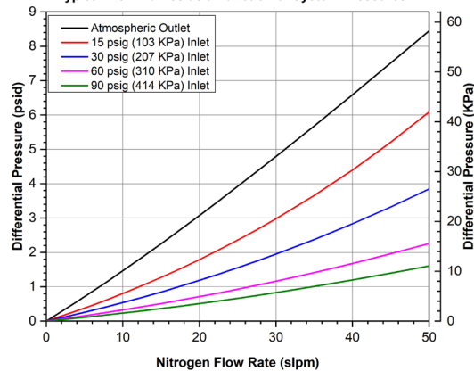
Mott GSMM-75-050-14 Flow Rate vs. Differential Pressure Typical Flow Curves as a Function of System Pressures
