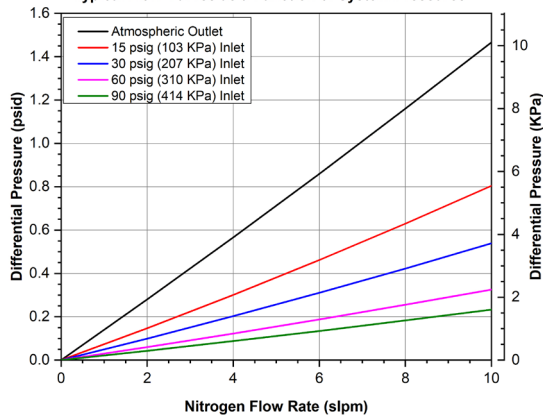
Mott GSMM-75-010-14 Flow Rate vs. Differential Pressure Typical Flow Curves as a Function of System Pressures
