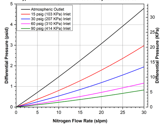
Mott GSMM-75-030-14 Flow Rate vs. Differential Pressure Typical Flow Curves as a Function of System Pressures
