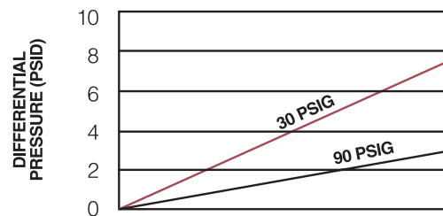
TYPICAL DIFFERENTIAL PRESSURE vs. FLOW
