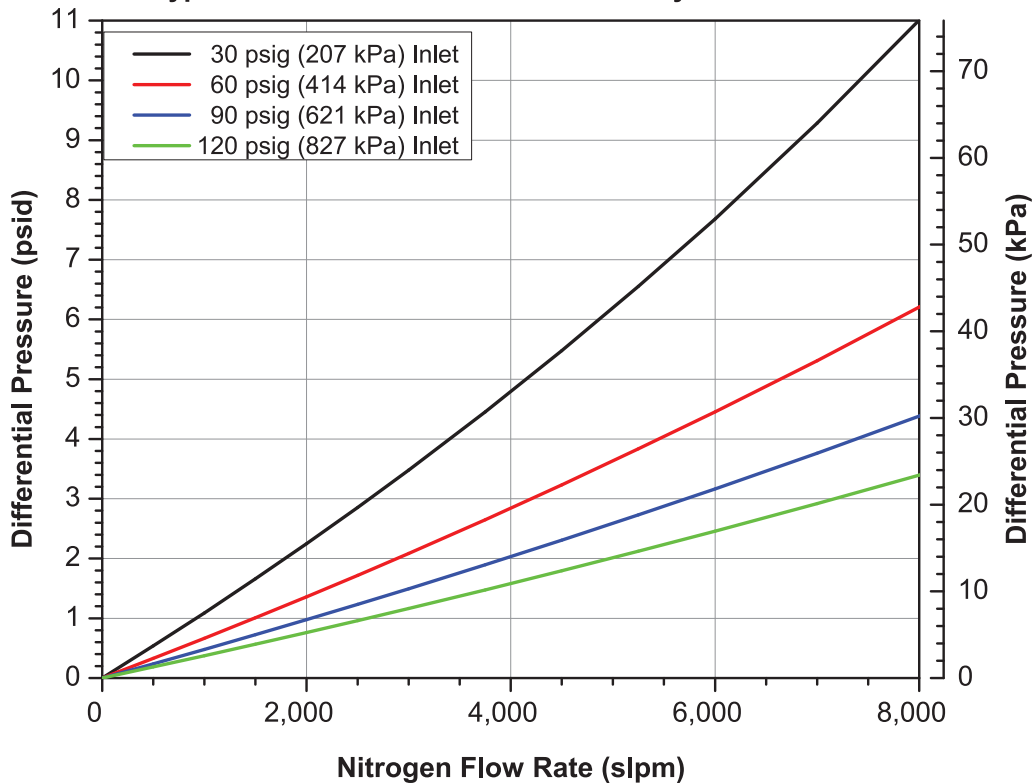
Mott BGF-315 Flow Rate vs. Differential Pressure Typical Flow Curves as a Function of System Pressures
